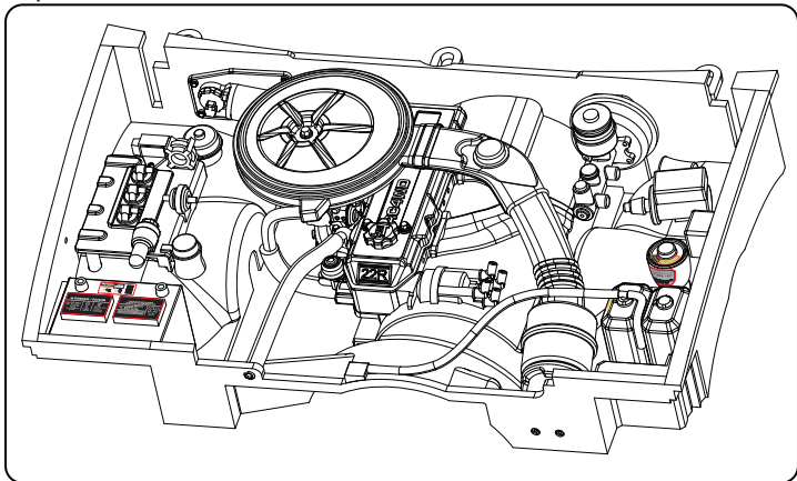
Step 30. DECAL INSTRUCTIONS.
